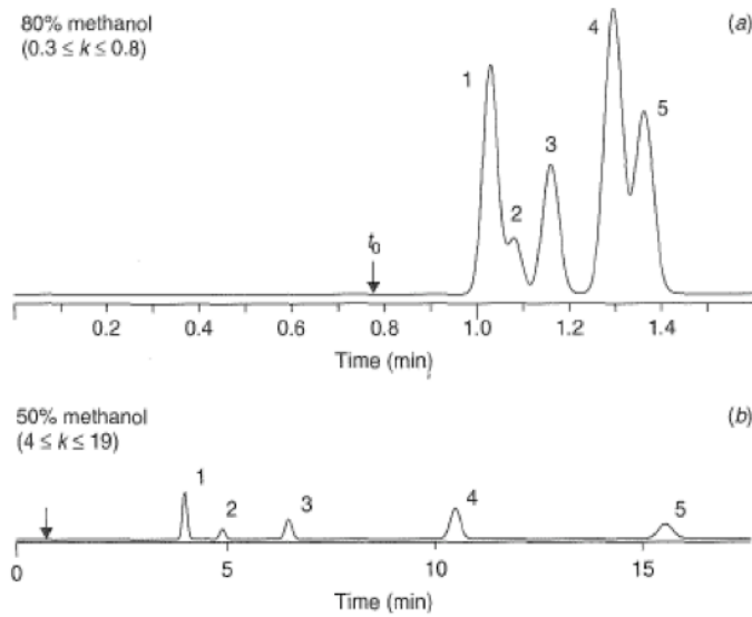
Figure 2.6 Separation as a function of mobile phase %B (%v methanol). Herbicide sample: 1, monolinuron; 2, metobromuron; 3, diuron; 4, propazine; 5, chloroxuron. Conditions, 150 × 4.6-mm, 5-μm C 18 column; methanol/water mixtures as mobile phase; 2.0 mL/min; ambient temperature. Recreated chromatograms from data of [7].
