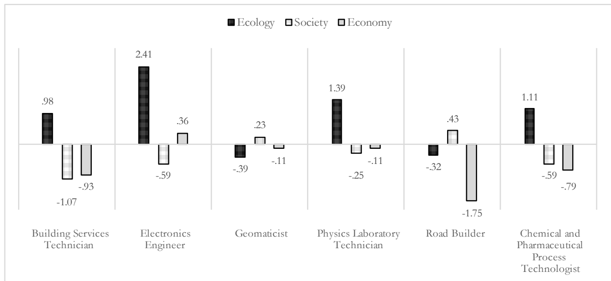
Fig. 2. z-standardized frequencies of SD dimensions by occupation (grand mean centered).
